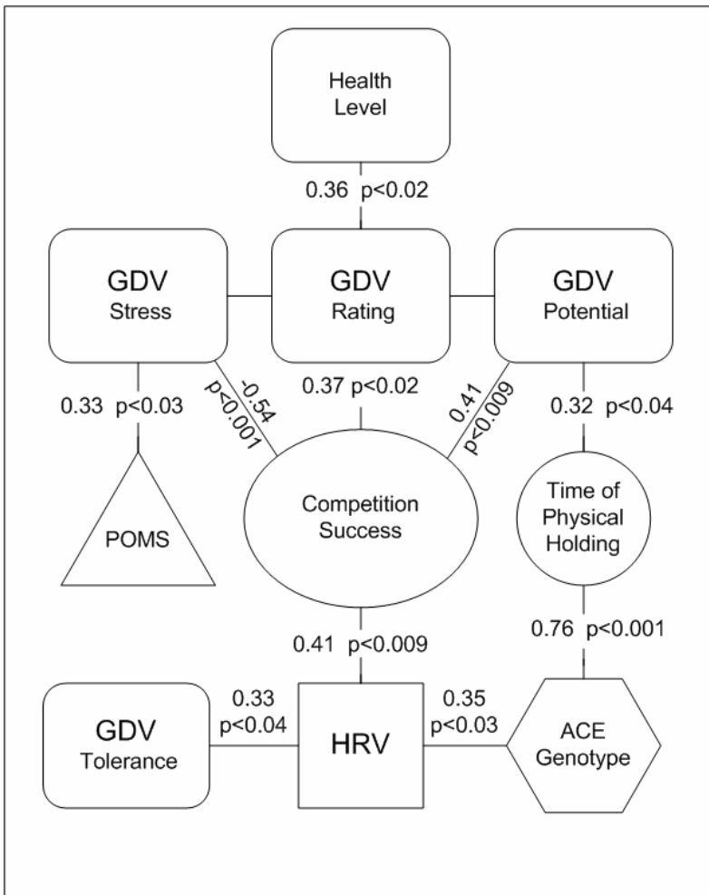
Fig. 4. Correlations between parameters in a group of 45 athletes. Spearman correlation coefficients are indicated.
