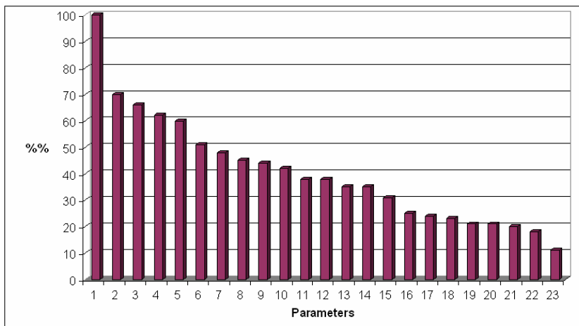
Fig. 5. Diagram of the correlation significance of various parameters relative to athletic success over two years in 196 athletes engaged in sports with high exercise loads.
